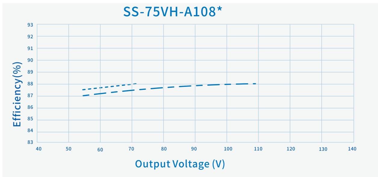
Efficiency Vs. Output Voltage (Vin=120Vac)
