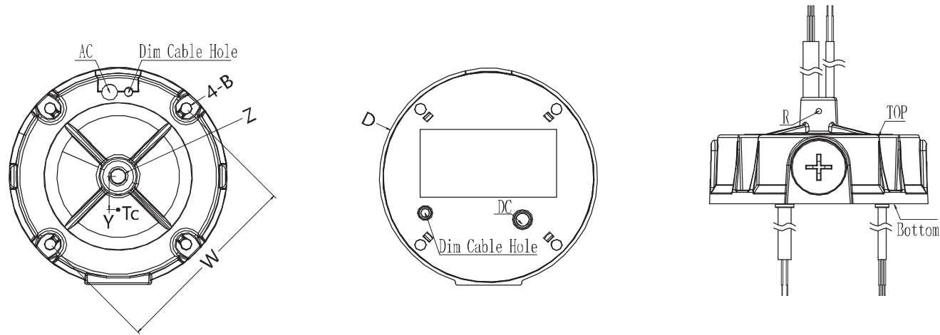
DIM cable from the bottom and top
