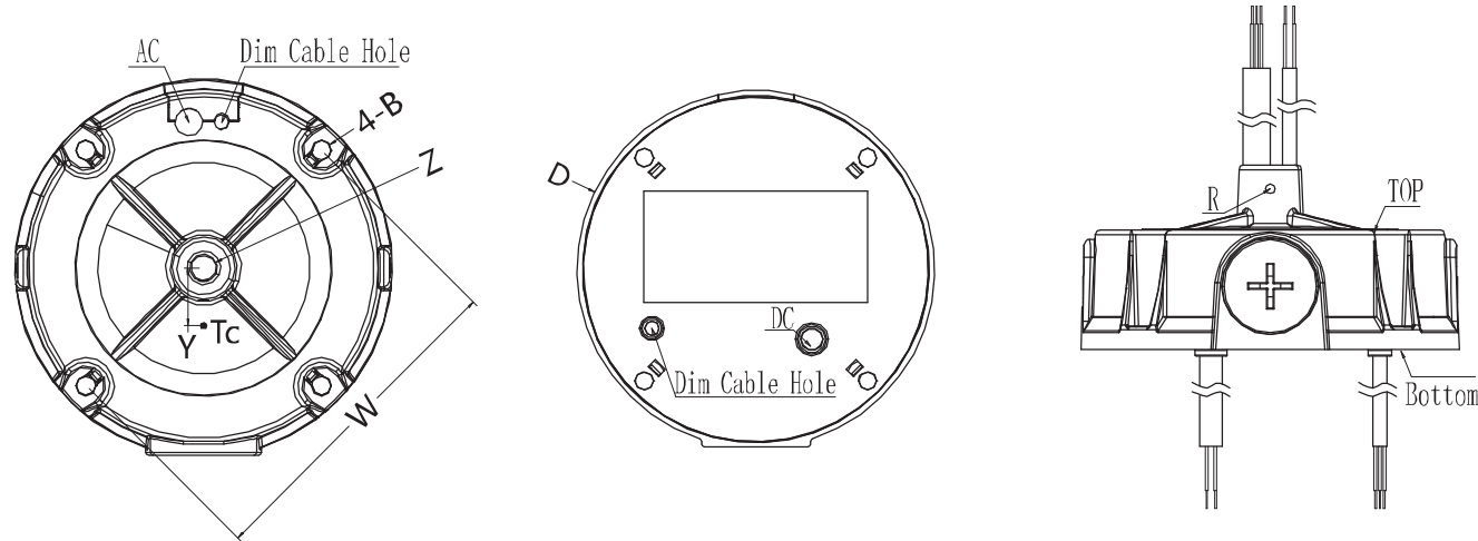
DIM cable from the bottom and top
