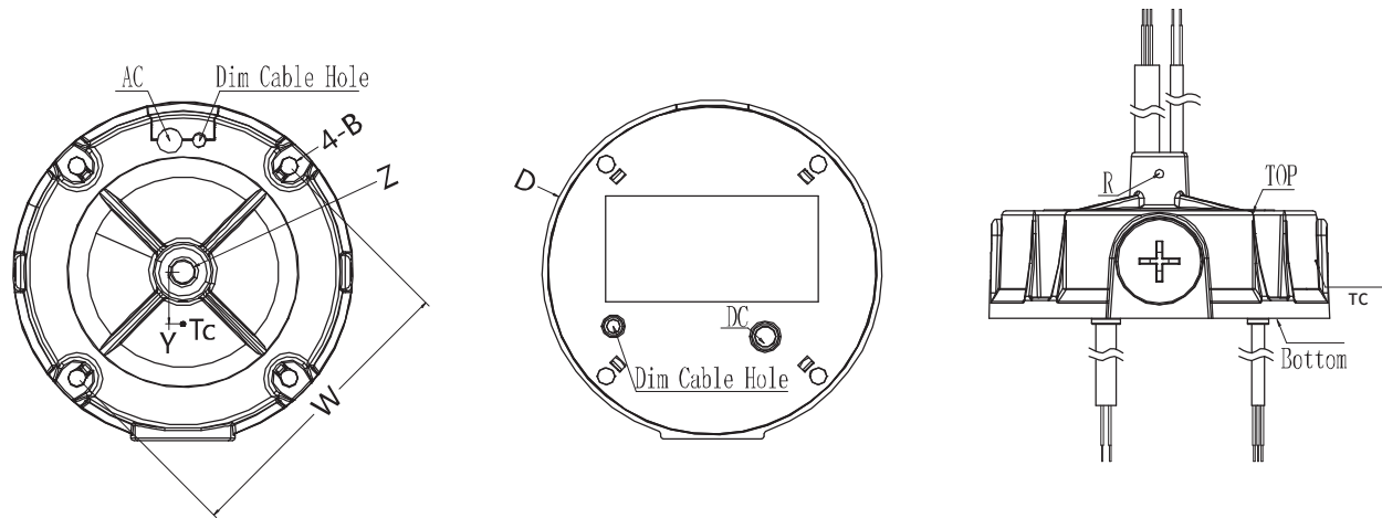
DIM cable from the bottom and top
