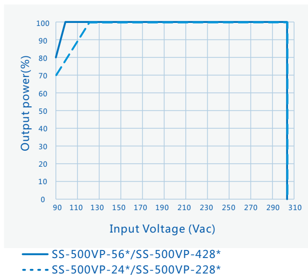
O/P Power Vs. Input Voltage
